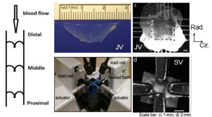
Fig. 1 Mechanical testing for JV and SV tissues
