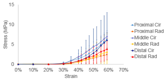
Fig. 2 JV stress-strain curves
