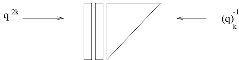
Figure 6: Computing the generating function for partitions with no '1' from the Ferrers diagram.
