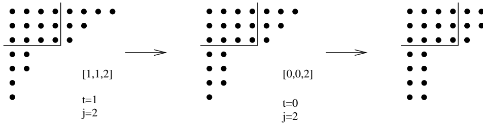
Figure 3: Computation of G((8, 6, 5, 2, 2, 1, 1)) , which uses case b(iii) of G .
